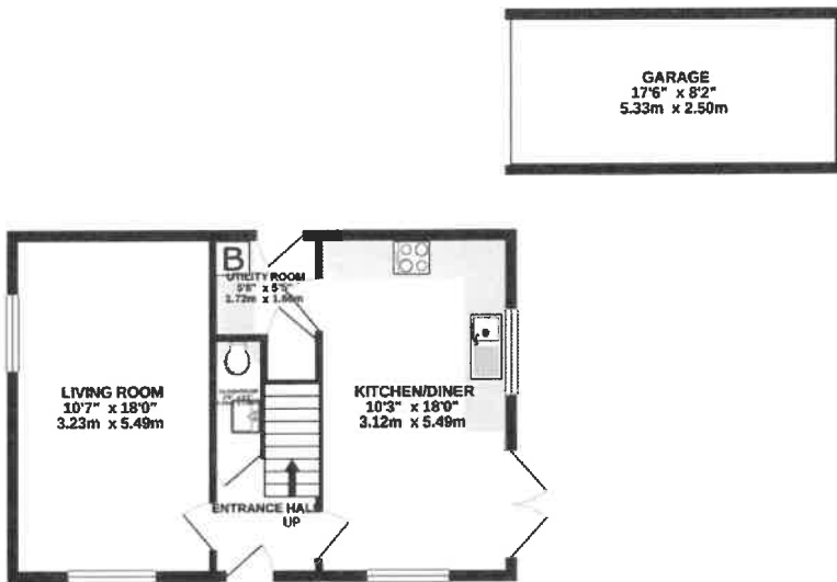
GROUND FLOOR 622 sq.ft. (57.8 sq.m.) approx.
