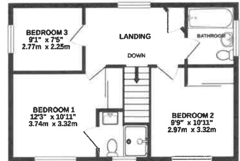
1ST FLOOR 479 sq.ft. (44.5 sq.m.) approx.
